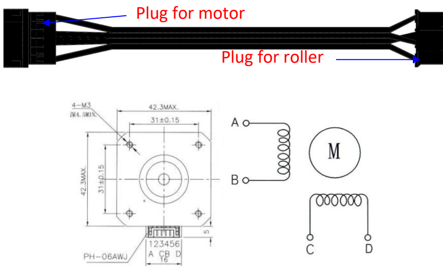
Motor Wire Sequence for Black Terminal Cables
